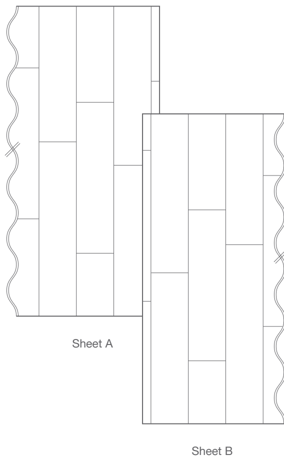
Diagram 2 – Both edges of the sheet have a narrow edge which needs to be trimmed to leave a full plank. Overlap sheet A over sheet B as indicated above and cut in the joint, cutting both sheets so that the join runs down the edge of the planks.
