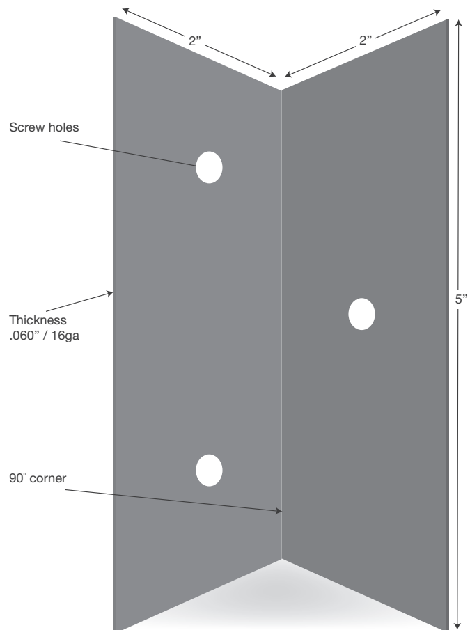
5" Stainless steel corner protector Interior view
