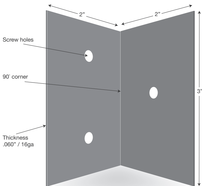
3" Stainless steel corner protector Interior view
