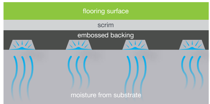
Enlarged to show cross-section construction of Altro Cantata
